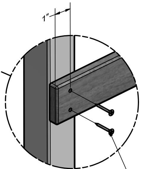
SCREW PFH 8x1 1/4 (2 PLCS)
