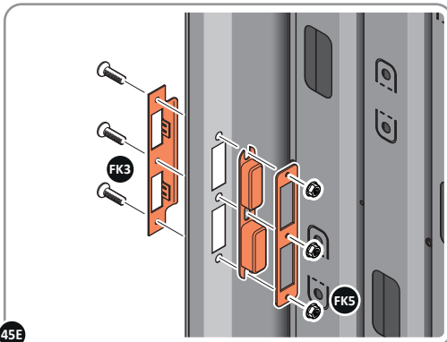
45E LOCATE AND SECURE EURO MORTICE LOCK 0203-32 AND CATCH PLATE COVER 0203-41 AS SHOWN ABOVE.
