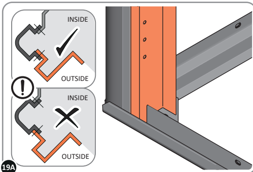
19A LOCATE RIGHT-HAND DOOR POST 0205-17 AS SHOWN ABOVE.
