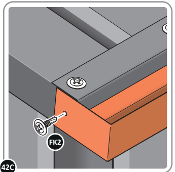
42C SECURE SLIDE ROOF GUTTER 0215-05 AT X2 LOCATIONS.
