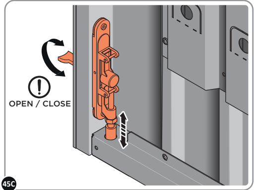
45C ENSURE FLUSH DOOR BOLT OPENS AND CLOSES.
