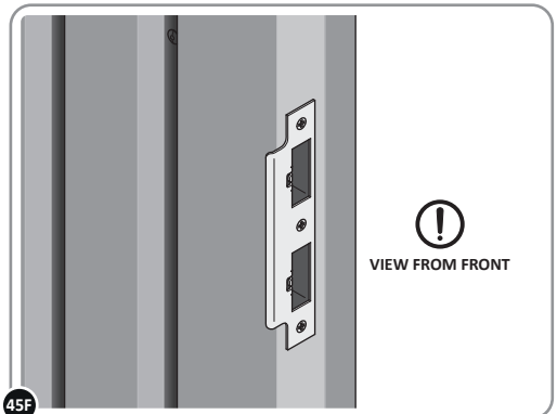
45F SECURED EURO MORTICE LOCK 0203-32 AS SEEN FROM FRONT.
