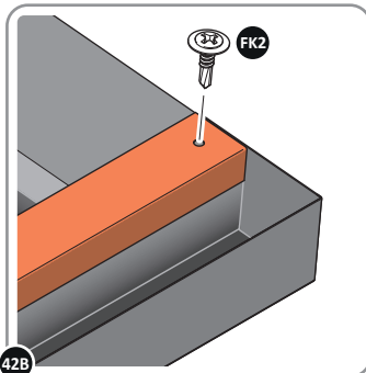
42B SECURE REAR ROOF CAP AT X8 LOCATIONS.
